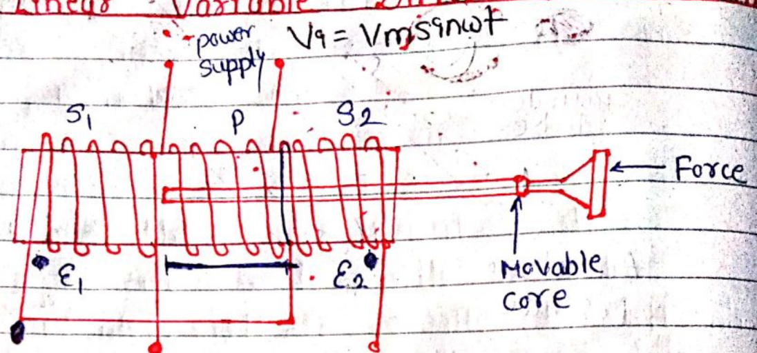
fig (a) Essential Component of LVDT
