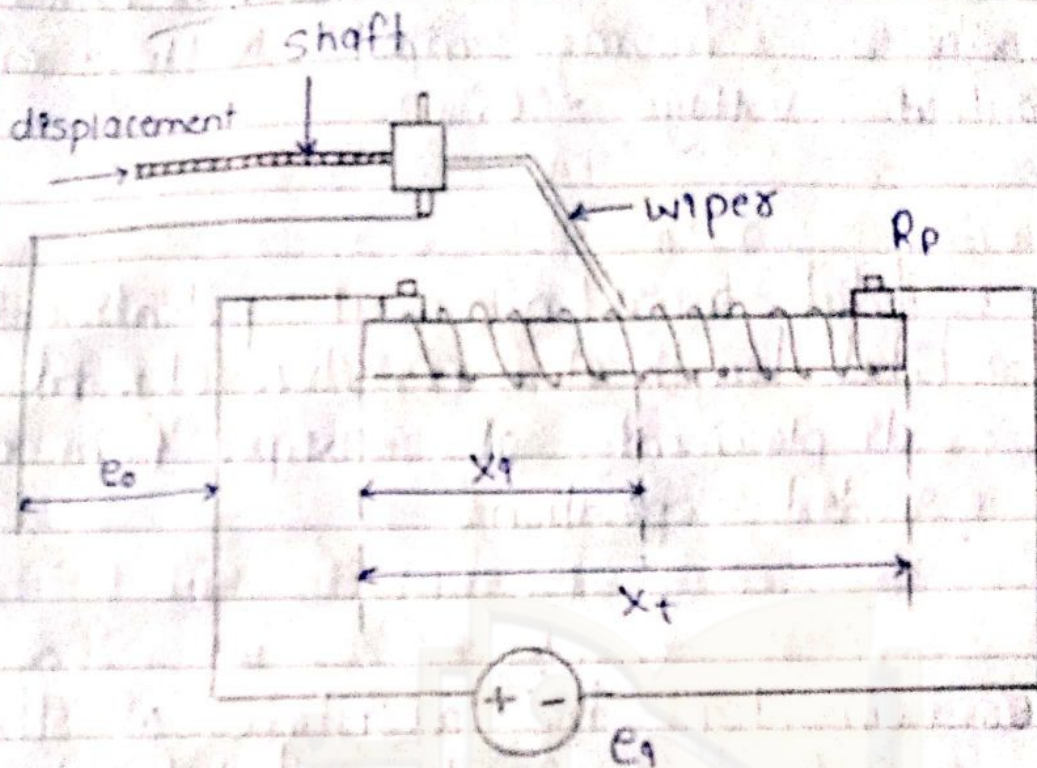
Fig: Linear potentiometer (a)
