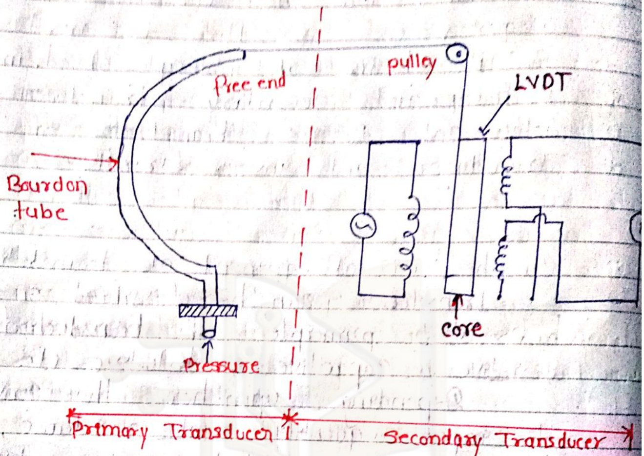
Fig: Measurement of pressure
